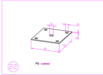
PD 40x40x1,0
