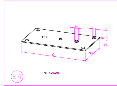
PD 80x40x1,0
