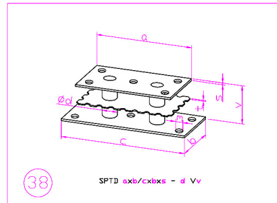
SPTD 50x25/65x25x1,0 - 8
