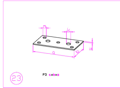
PD 50x25x1,0
